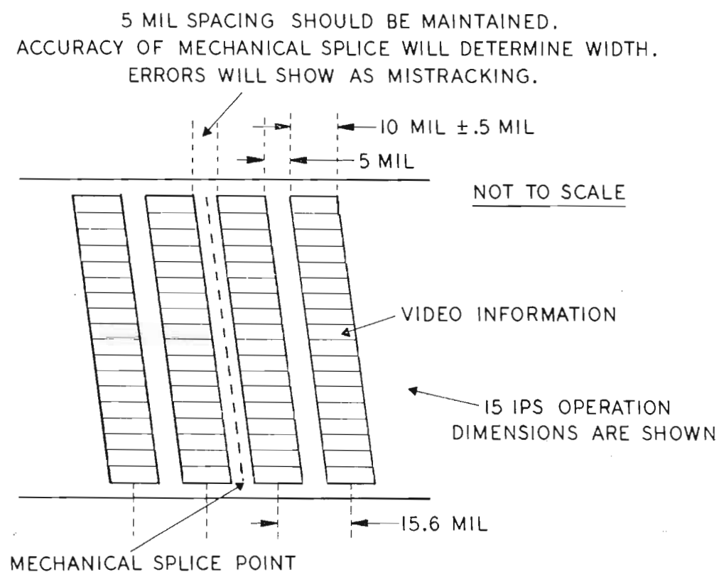
FIG. 7 Diagram showing track spacing tolerances and likely effects of mechanical splice. Electronic splicing does not affect track spacing at the splice point.
