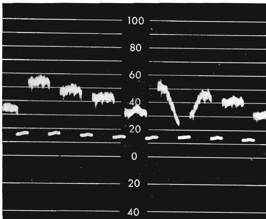
FIG. 5 FM switcher output waveform (SW OUT) on CRO with ERASE TEST button held down (High Band machine).
