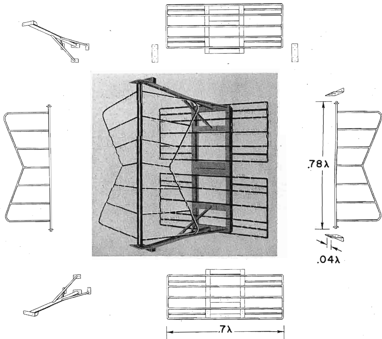
FIG. 1 Test Model of the "Butterfly" Antenna made up of three panels mounted around a triangular tower structure. Optimum impedance and radiation characteristics are achieved by positioning the "wings" backward.
