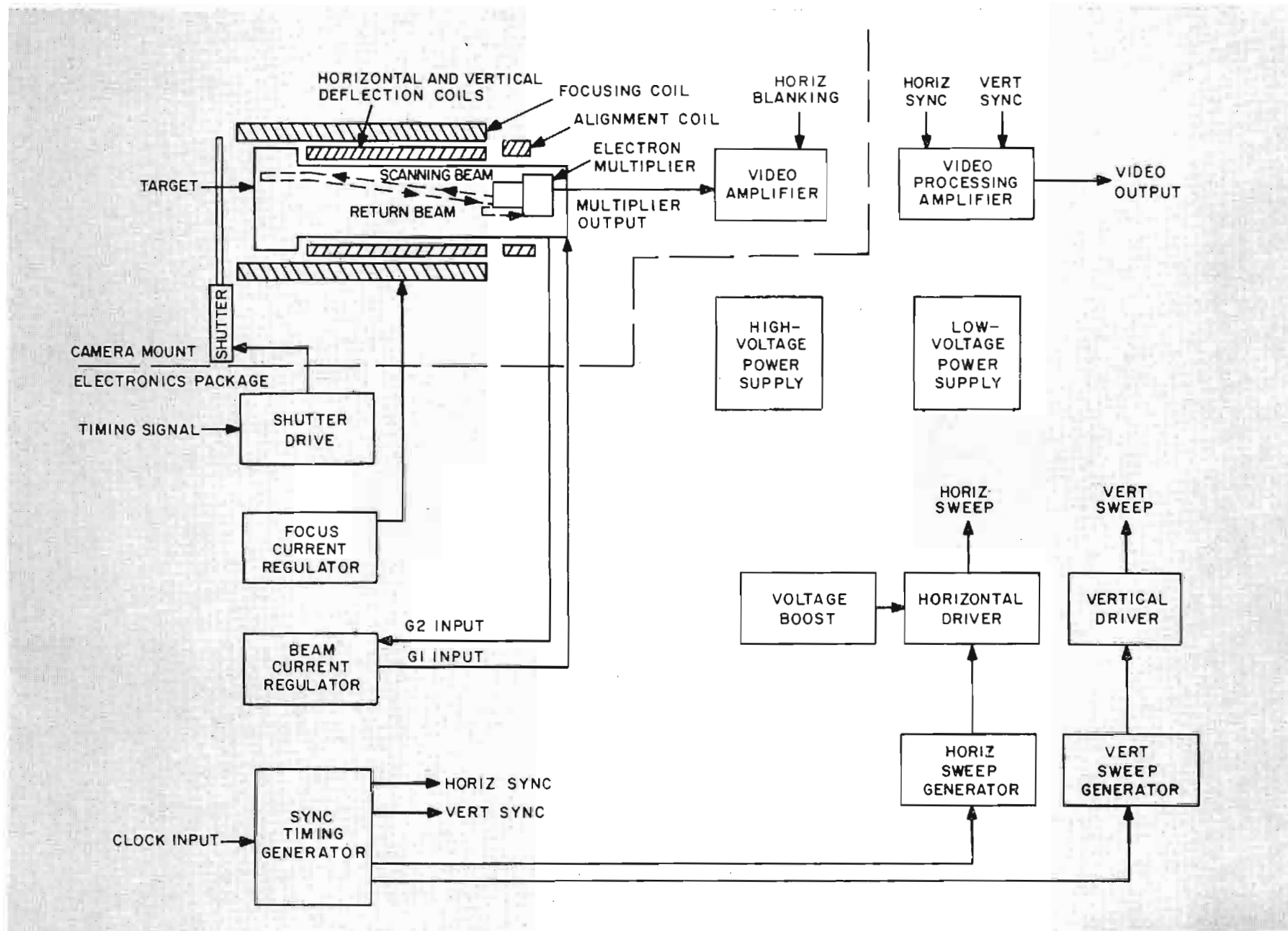
FIG. 4 Simplified Block Diagram of Return Beam Vidicon.
